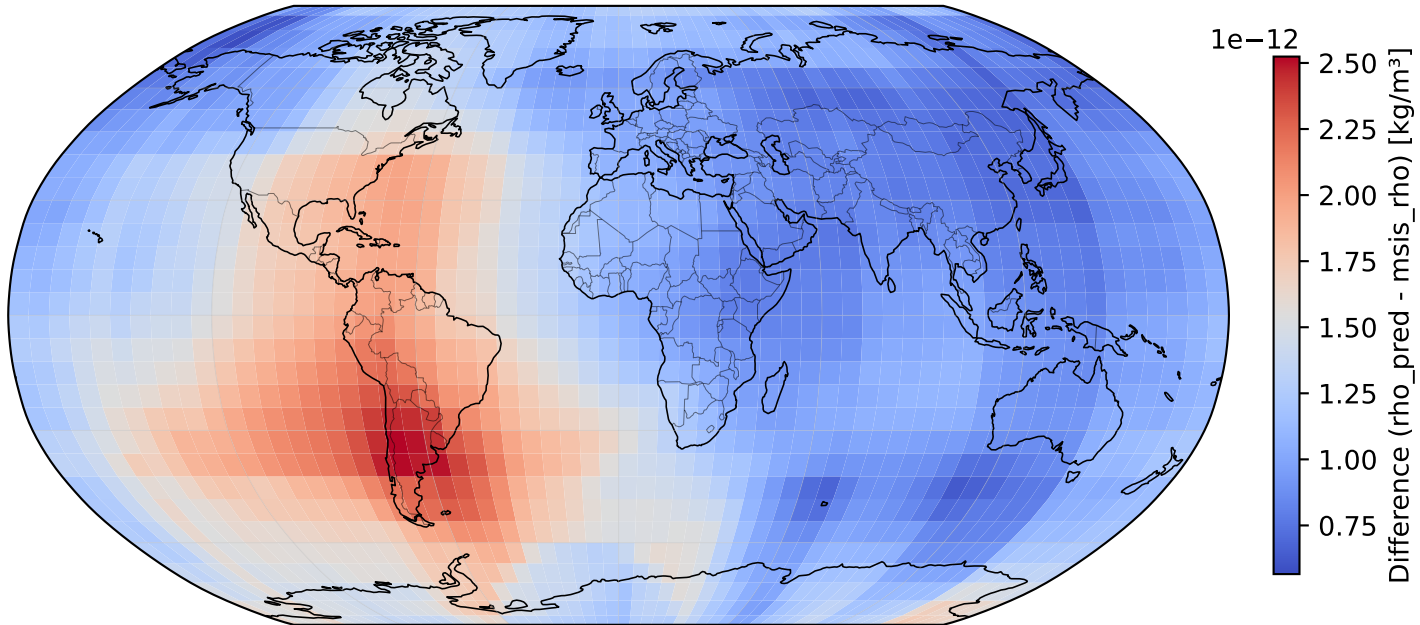
ML model – NRLMSIS-2.1
