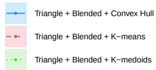
Clustering Method
