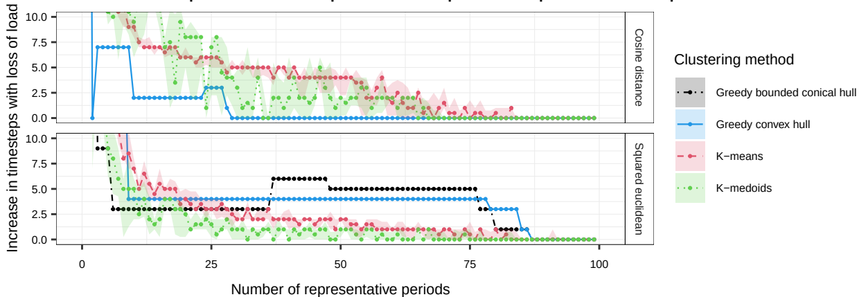
Increase in timesteps with loss of load per number of representative periods – 2D example
