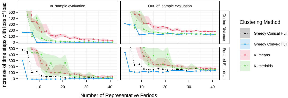
Increase in loss of load for different number of Representative Periods – Separate clusters with spatial correlation
