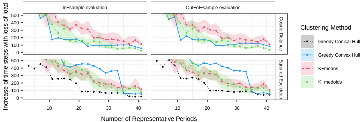
Increase in loss of load for different number of Representative Periods – Separate clusters without spatial correlation
