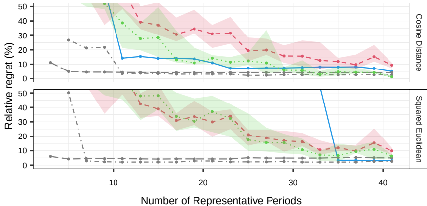
Relative regret for different number of Representative Periods – Separate clusters without spatial correlation
