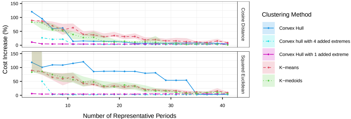
Cost Increase % for different number of Representative Periods – Separate clusters without spatial correlation
