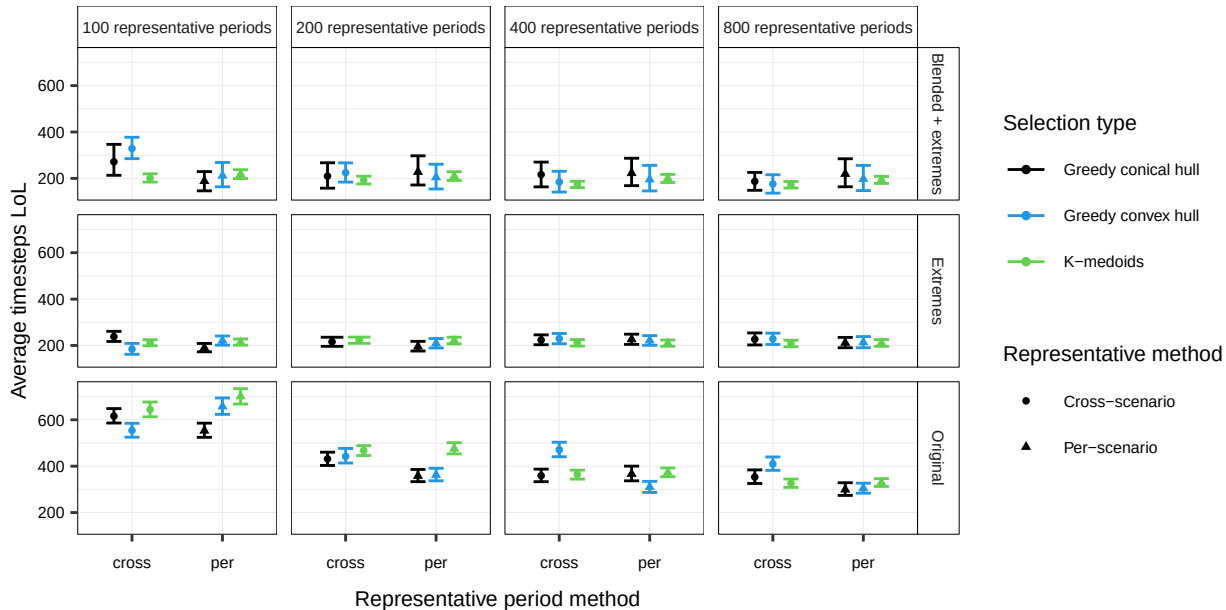
Average number of timesteps containing LoL over in-sample scenarios
