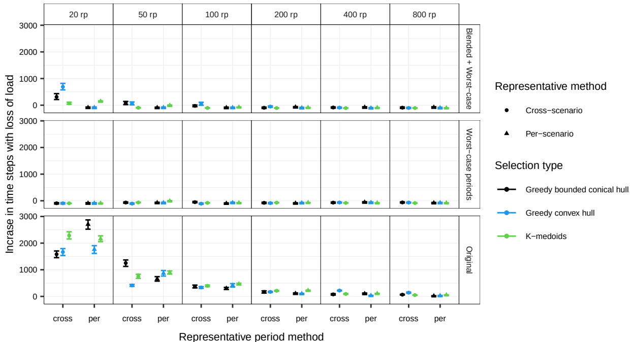
Average increase in time steps with loss of load over all out-of-sample scenarios
