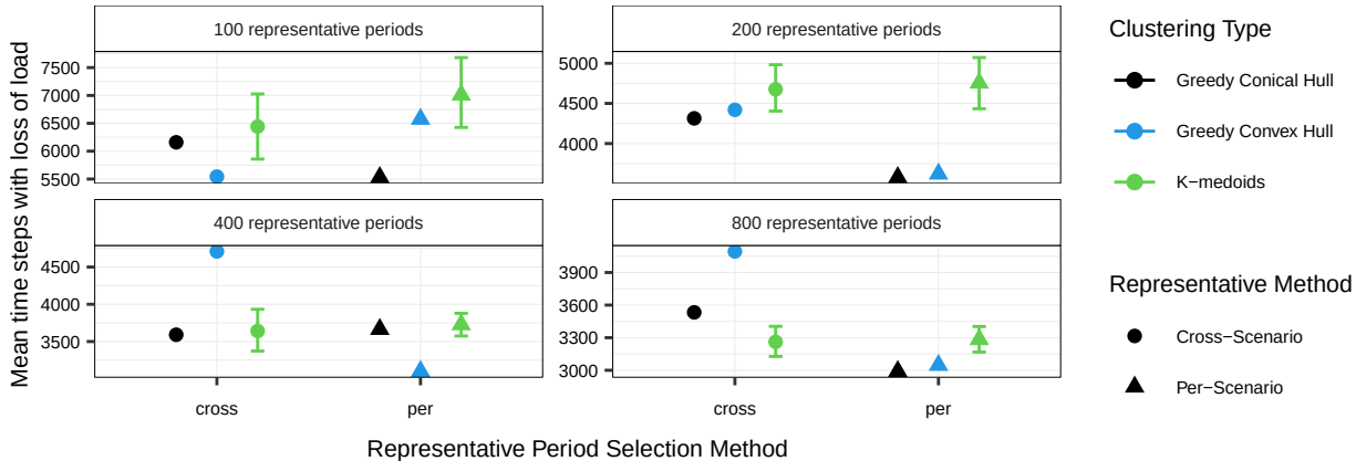
Number of time steps with loss of load
