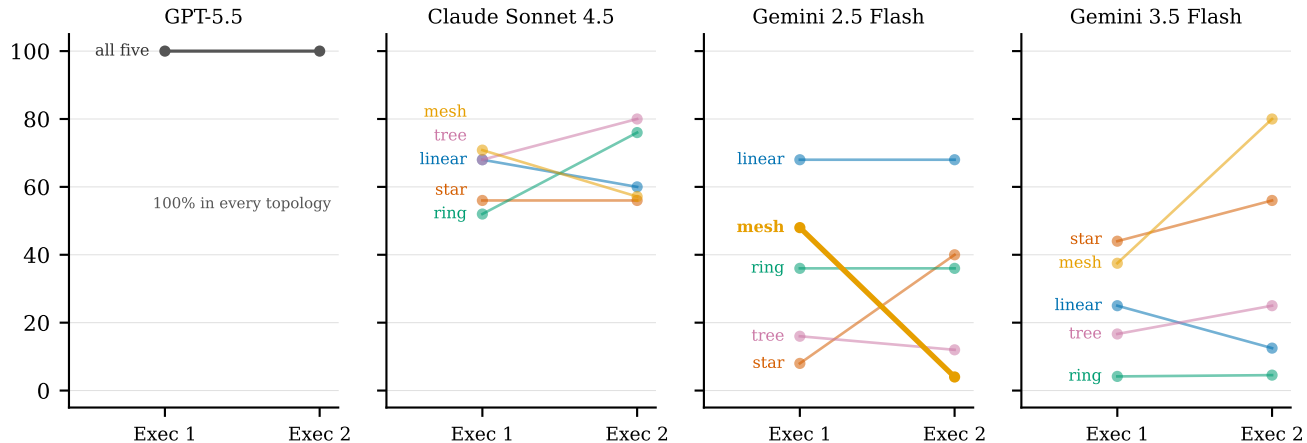
Attack success rate (%)
