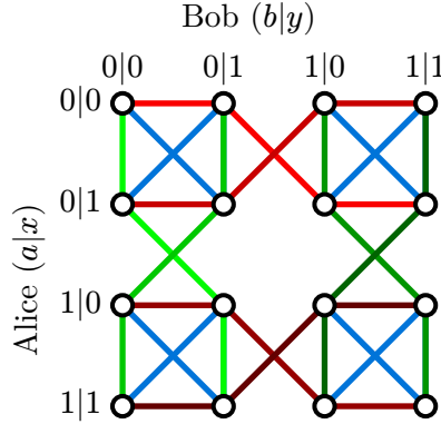
Figure 2: Contextual hypergraph of the Bell (2, 2, 2) scenario. The hyperedges are represented by the same color.
