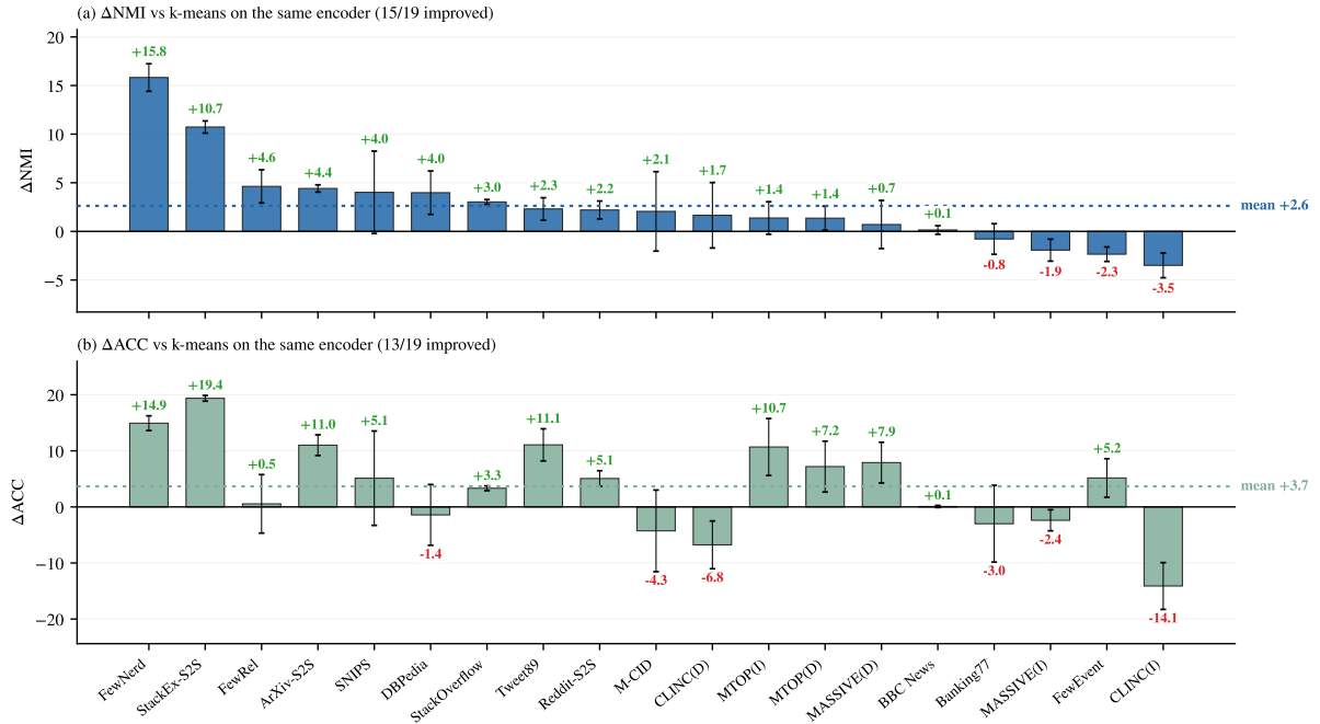
Figure 8: Improvement of CLEAR over k-means on the same encoder, seed-paired per run, for (a) NMI and (b) ACC (gemini-embedding-001 embeddings, glm-5 as the LLM). Bars are mean deltas over the five runs. Whiskers show one standard deviation over the 5 runs, and the dotted lines show the mean over the 19 benchmarks.
