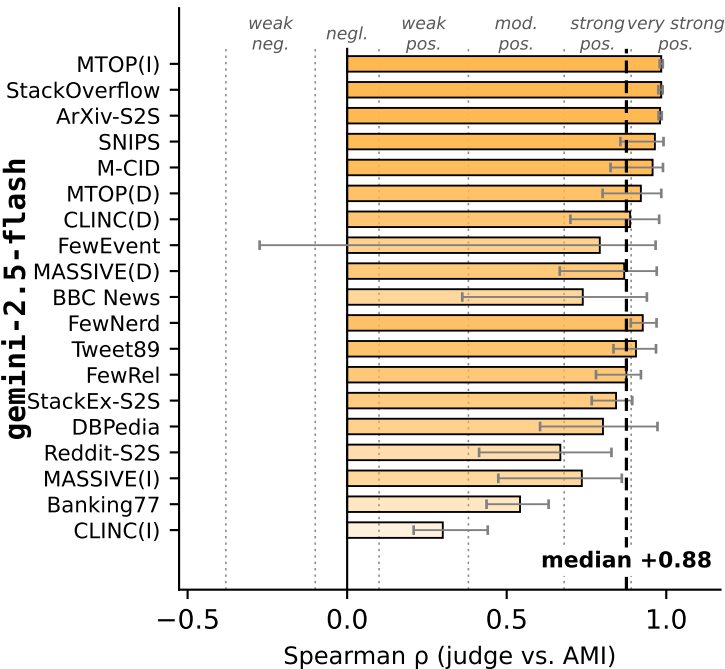
Judge-AMI correlation per benchmark
