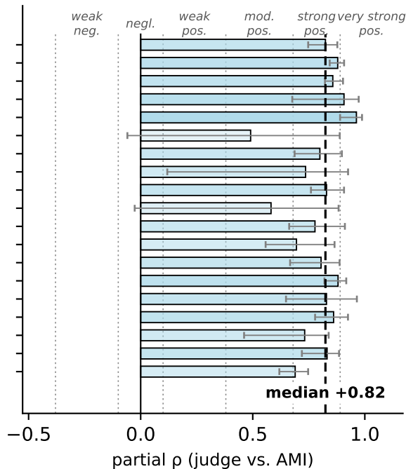
Controlling for silhouette + Caliński-Harabasz jointly
