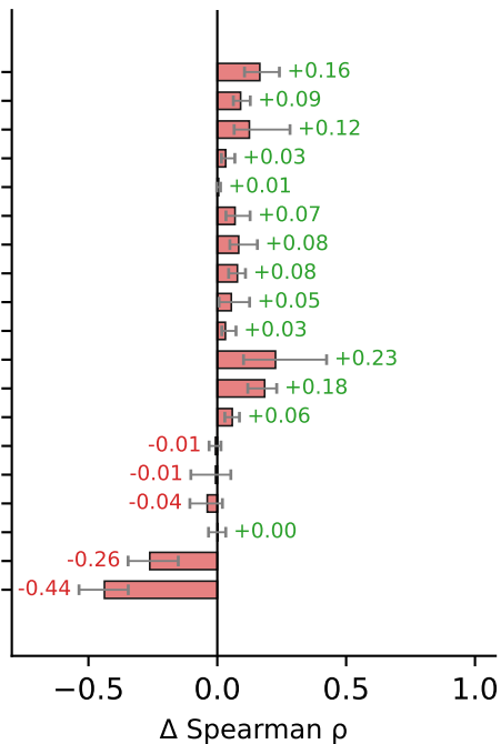
Gap between the two (raw – controlled)
