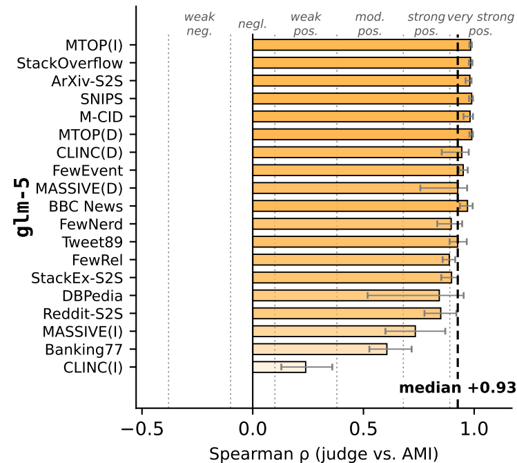
Judge-AMI correlation per benchmark
