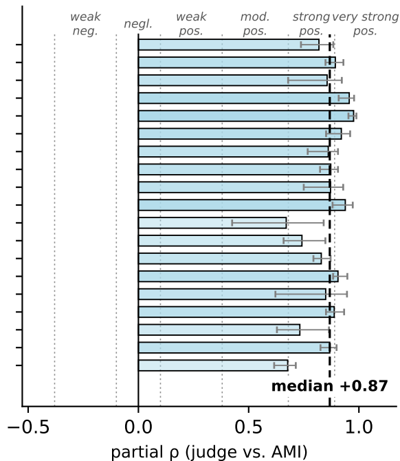
Controlling for silhouette + Caliński-Harabasz jointly
