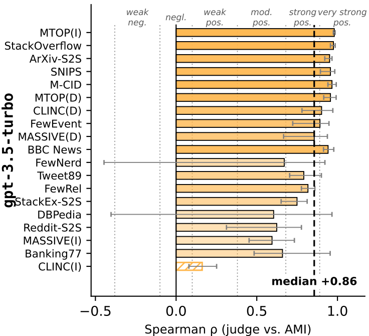
Judge-AMI correlation per benchmark
