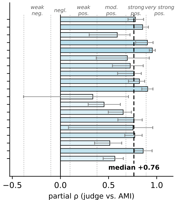
Controlling for silhouette + Caliński-Harabasz jointly
