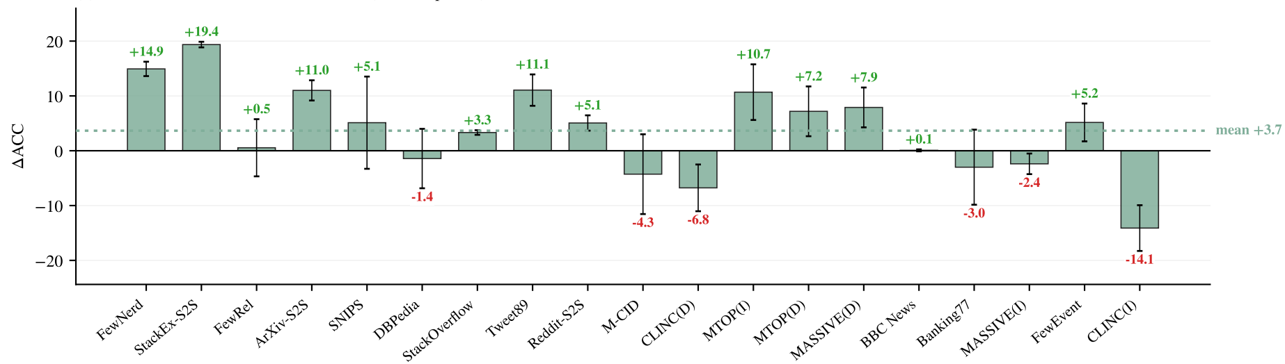
(b) \Delta ACC vs k-means on the same encoder (13/19 improved)
