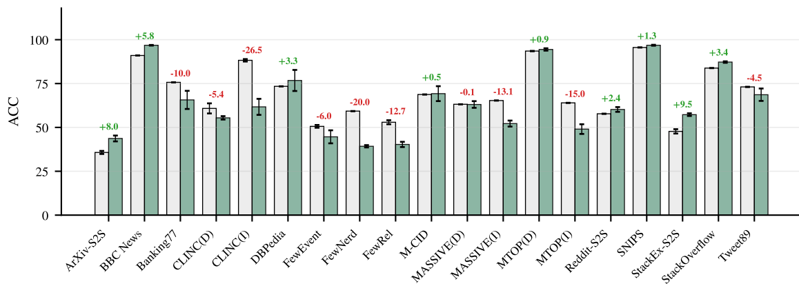
(d) matched, ACC: ahead of the best published result on 9/19
