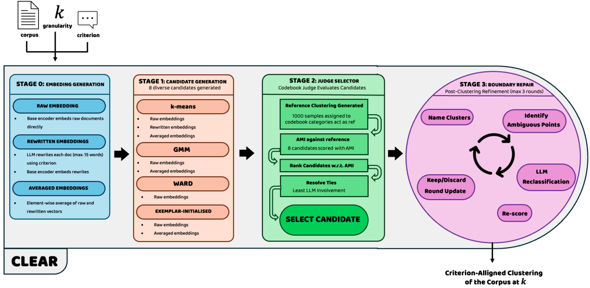
Figure 4: Overview of the three-stage CLEAR pipeline. The inputs in the top-left are the original raw corpus, the choice of granularity, and the clustering criterion. Output on the bottom-right is the criterion-aligned clustering of the corpus at k
