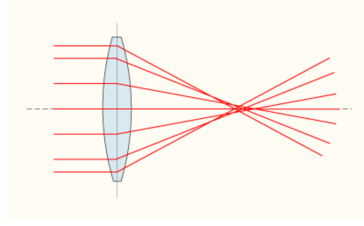
FIGURE 1.2 – aberration sphérique
