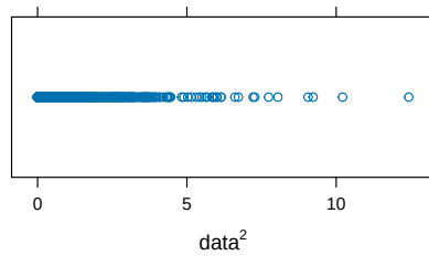
(c) Stripplot
