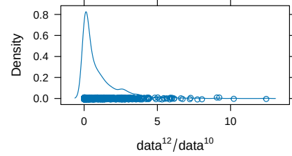
(b) Densityplot
