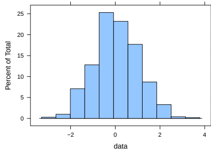
(a) Histogram
