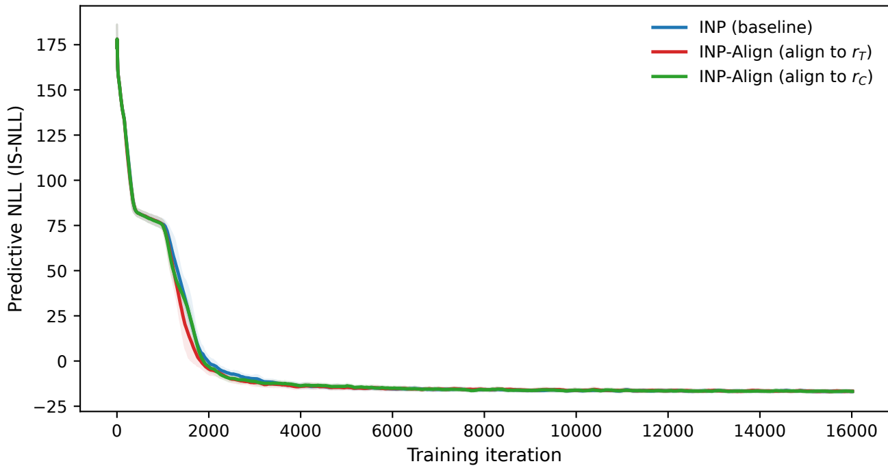
Training predictive NLL
