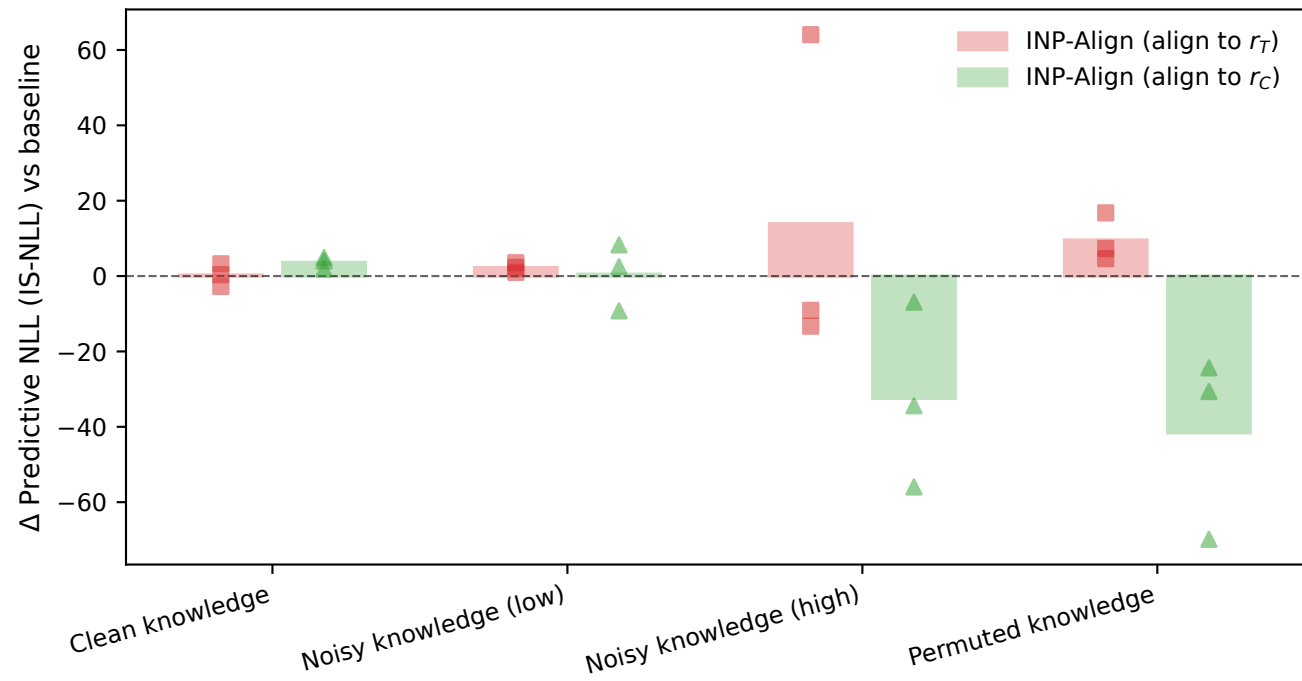
Robustness: \Delta NLL relative to INP (baseline)
