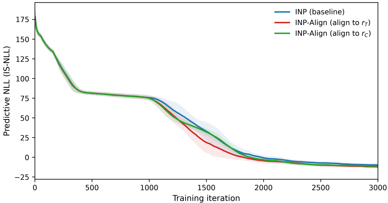
Training predictive NLL (early iterations)
