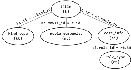
Figure 1: A join pattern in the IMDB schema [38].
