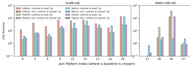
Figure 7: Log-scale running time per join pattern (where a baseline is chosen) in scale and stats_ceb, including HYBRID’s.
