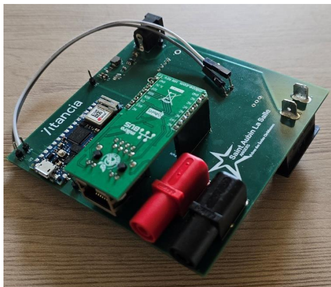
Figure 21 PCB final
