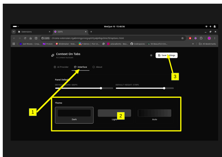
Figure 8: Theme setup
