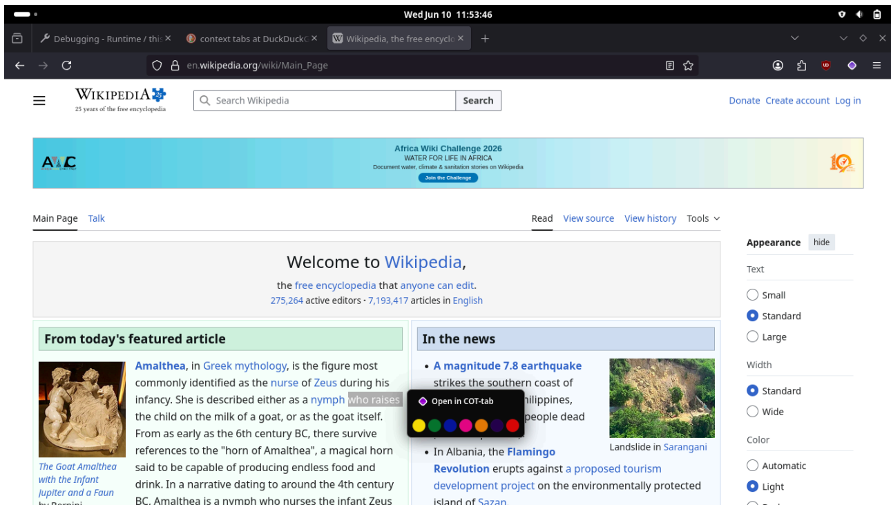
Figure 9: Tooltip
