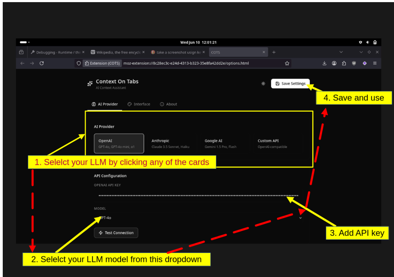
Figure 7: LLM Setup
