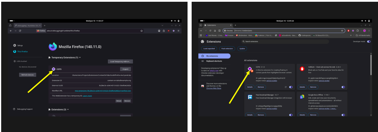
Figure 3: Listed Extensions
