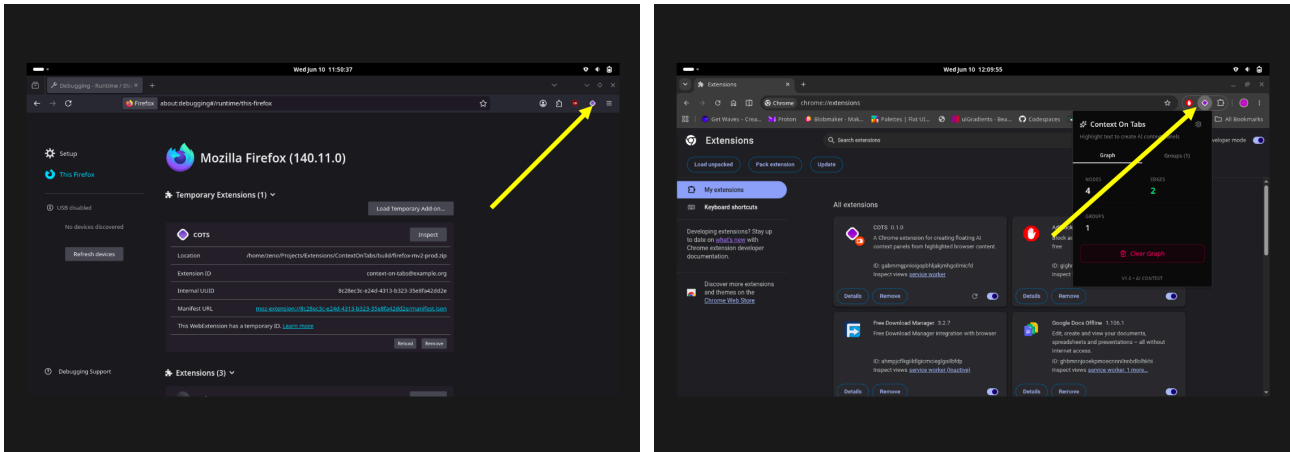
Figure 5: Pinned Extensions
