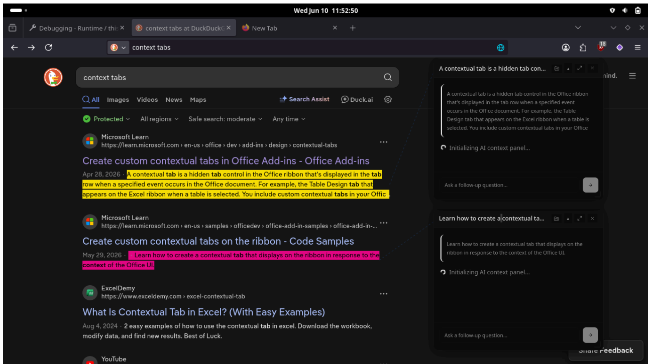
Figure 11: Tooltip
