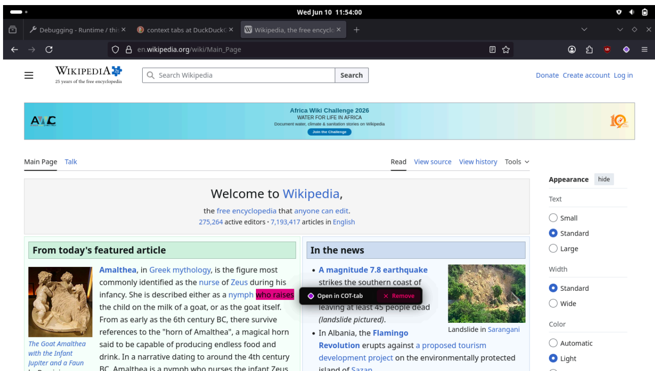
Figure 10: Tooltip
