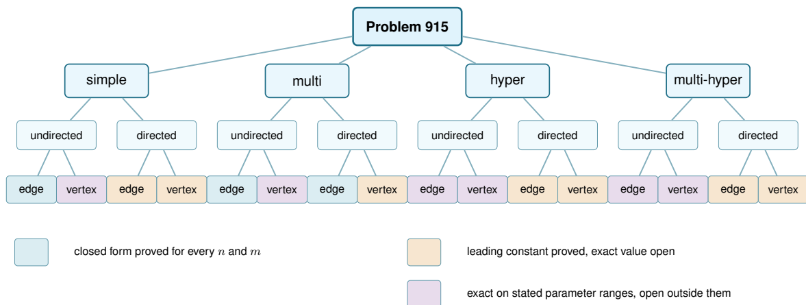
Figure 3.3. Status of the sixteen variants. Blue marks a closed form proved for every n and m . Purple marks an exact value proved on stated parameter ranges and open outside them. Amber marks a proved leading term with the general exact value unknown. For simple directed arcs, Conjecture 3.1 concerns only sufficiently large orders. The model and direction rows carry no status. Table 3.1 is authoritative for exceptions and conventions.
