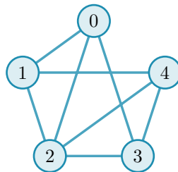
Figure 1.1. A simple graph on five vertices. It is K_5 , the complete graph in which every one of the \binom{5}{2} = 10 pairs is joined by an edge, with the two edges \{0, 4\} and \{1, 3\} removed, so its edge set E(G) holds eight edges. The five dots are the vertex set V(G) and the lines are the edges. Because at most one line joins any given pair and no edge loops back to its own endpoint, this is a simple graph. The same graph returns in Figure 1.2 , once we can count the independent routes between a pair.
