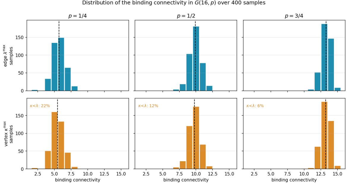
Figure 1.11. Distributions of the binding connectivity in G(16, p) over 400 samples, at densities p = \frac{1}{4}, \frac{1}{2}, \frac{3}{4} . The top row histograms the edge-connectivity \lambda^{\max} , the bottom row the vertex-connectivity \kappa^{\max} , measured on the same samples, with the mean marked by a dashed line and the fraction of samples on which \kappa^{\max} < \lambda^{\max} printed on each vertex panel. Reading a column top to bottom, the vertex distribution sits at or to the left of the edge one, which is Whitney's inequality, and the gap is largest at the sparsest density (22% of samples) and closes as p grows (6%). All six panels share one axis range.
