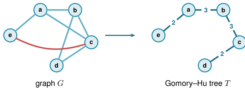
Figure A.1. A simple graph G (left) and a Gomory–Hu tree T of it (right). Both live on the same five vertices, and here T is the path e-a-b-c-d with the marked cut weights. The four edges ea, ab, bc, cd are also tree edges, so each has \text{dist}_T(e) = 1 : these are the E_1 edges of Lemma A.4 , and a simple graph admits at most n-1 = 4 of them, one per tree edge. The edges ac and bd join tree-distance-2 pairs, and the red chord ec has \text{dist}_T(ec) = 3 , crossing all three cuts on the path e-a-b-c . Reading \text{dist}_T(e) as the number of tree cuts an edge crosses makes \sum_e \text{dist}_T(e) = \sum_t c(t) ( Lemma A.6 ). Every edge crosses at least one cut, but only the n-1 tree edges cross exactly one, which is the surplus that drives Lemma A.5 and ultimately the factor of two in Mader’s bound.
