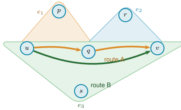
Figure 1.10. Two Berge routes between u and v that share no hyperedge. Route A (orange) threads e_1 then e_2 , hopping hyperedge at q , and route B (green) crosses the single hyperedge e_3 . The two use disjoint hyperedge sets \{e_1, e_2\} and \{e_3\} , so they are Berge edge-disjoint and \lambda(u, v) \geq 2 . Any third route would have to reuse one of the three hyperedges. This is the hypergraph form of edge-disjoint routes, with a whole hyperedge, not a single edge, consumed by each route.
