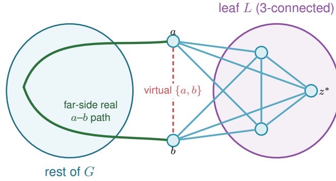
Figure A.7. The triconnected (Tutte/SPQR) decomposition in Step 4 of Lemma A.40, schematic: G splits into a tree of pieces (blobs) glued along virtual edges, and the analysis works at a leaf L with its single virtual edge \{a, b\} (dashed red). The far side of the tree supplies a real a - b path (green) that internally avoids L . If L is 3-connected, any two of its vertices are joined by three internally disjoint paths inside L , at most one using the virtual edge, and the far-side path replaces it, so \kappa_G \geq 3 for every pair in L . With |V(L)| \geq 4 that forces a hyperedge-node z^* \notin \{a, b\} of degree at most one, which is the contradiction that closes the lemma.
