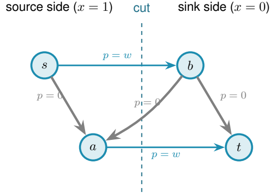
Figure 2.6. One ordered pair's chosen cut. The dashed line splits the vertices into the source side, where x_u^{st} = 1 , and the sink side, where x_u^{st} = 0 . Only arcs running from source side to sink side cross the cut, and the first constraint forces their helper p_{uv}^{st} up to the arc weight w (the two thick arcs). Arcs that stay on one side, and arcs that run the other way across the line, contribute nothing. The second constraint then caps the total counted weight, the thick arcs, at one.
