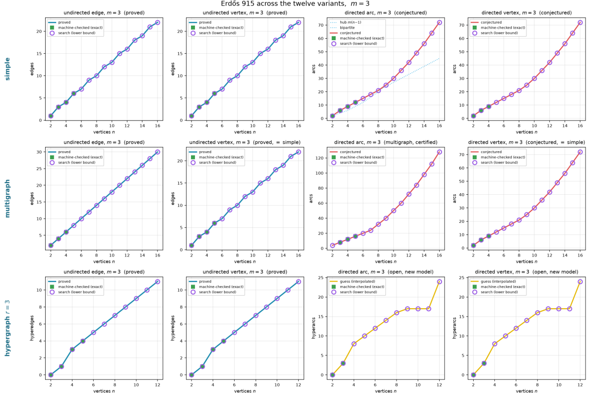
Figure 3.5. All twelve variants at m=3 , edges against n , laid out by model (rows: simple, multigraph, 3-uniform hypergraph) and by separation and direction (columns: undirected edge, undirected vertex, directed arc, directed vertex). A blue curve is a value proved for all n , a red curve a conjectured formula, and a yellow curve a bare interpolation of the machine points where no formula is known, the three told apart by colour rather than by dash pattern. Filled squares are the sizes solve proved or certified exactly. Open circles are lower bounds at larger n , the better at each size of the search's densest find and a named construction measured by the checker, reported as a running maximum so a feasible graph at one size is never lost at the next. On the open variants the yellow curve is the piecewise-linear interpolation through those circles, never above them, and the axes are scaled to the data rather than to a loose certain interval. The directed hypergraph panels in the bottom row rise steeply because their value is quadratic in n , not linear.
