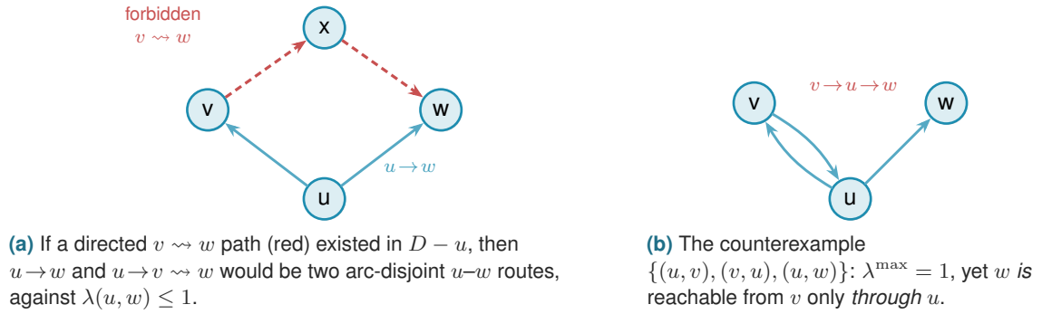
Figure A.2. Why Proposition A.25 must exclude paths through u . (a) For out-neighbours v, w of u in a digraph with \lambda^{\max} \leq 1 , no v \rightsquigarrow w path can avoid u : such a path would combine with the lone arc u \rightarrow w into two arc-disjoint routes. (b) The restriction to D - u is essential. In the three-vertex digraph \{(u, v), (v, u), (u, w)\} we have \lambda^{\max} = 1 , yet v reaches w via v \rightarrow u \rightarrow w , a route that reuses the vertex u , which the proposition allows.
