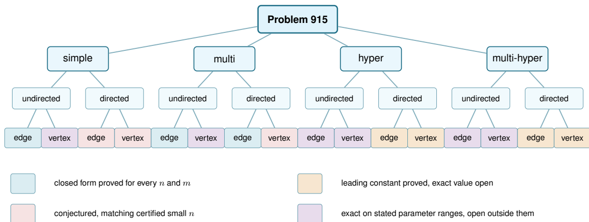
Figure 3.3. Status of the sixteen variants. Colour marks the status of a leaf: blue a closed form proved for every n and m , purple an exact value proved on stated parameter ranges and open outside them, red a conjectured exact formula with a proved lower bound, and amber a proved leading term with the exact value unknown. The model and direction rows are labels and carry no status, since each of them now covers two leaves that differ. Table 3.1 is authoritative for exceptions and conventions.
