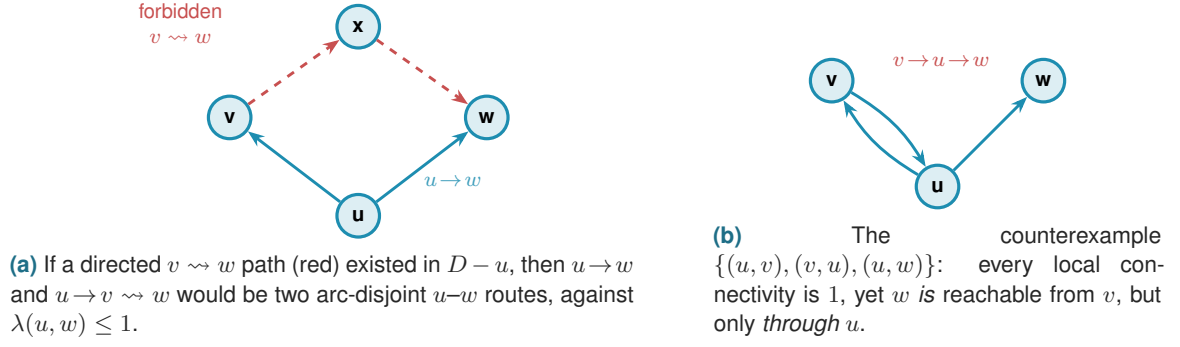
Figure A.3. Why Proposition A.16 must exclude paths through u . (a) For out-neighbours v, w of u in a digraph with \lambda_D^{\max} \leq 1 , no v \rightsquigarrow w path can avoid u : such a path would combine with the lone arc u \rightarrow w into two arc-disjoint routes. (b) The restriction to D - u is essential. In the three-vertex digraph \{(u, v), (v, u), (u, w)\} all connectivities equal 1, yet v reaches w via v \rightarrow u \rightarrow w , a route that reuses the vertex u , which the proposition allows.
