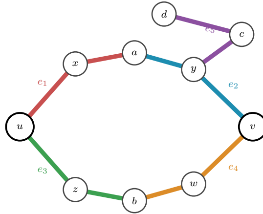
Figure 1.11. A three-uniform hypergraph on ten vertices, its five hyperedges drawn as metro lines. To travel from u to v one rides a line and changes at a shared station. Route A takes the red line e_1 to a and changes there to the blue line e_2 into v ; route B takes the green line e_3 to b and changes to the orange line e_4 . The two journeys share no line, so they are hyperedge-disjoint Berge routes and \lambda(u, v) \geq 2 . A third route would have to reuse a line already taken. Just as a metro line carries one train past a point at a time, a whole hyperedge, not a single edge, is what each route consumes.
