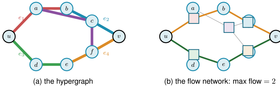
Figure 2.6. From hypergraph to flow network, before and after. (a) A hypergraph on eight vertices, its five hyperedges drawn as metro lines. The pair u, v has two hyperedge-disjoint Berge routes, u, e_1, b, e_2, v and u, e_3, e, e_4, v . (b) The same vertices with one helper square per hyperedge (a turnstile on each line). Each Berge route becomes a flow path that enters a line through one member, crosses its helper, and leaves through another: u \rightarrow h_{e_1} \rightarrow b \rightarrow h_{e_2} \rightarrow v (orange) and u \rightarrow h_{e_3} \rightarrow e \rightarrow h_{e_4} \rightarrow v (green). Because every helper carries only one unit, the maximum u-v flow is exactly two, which the checker reports as \lambda(u, v) = 2 . A third route would have to reuse a helper.
