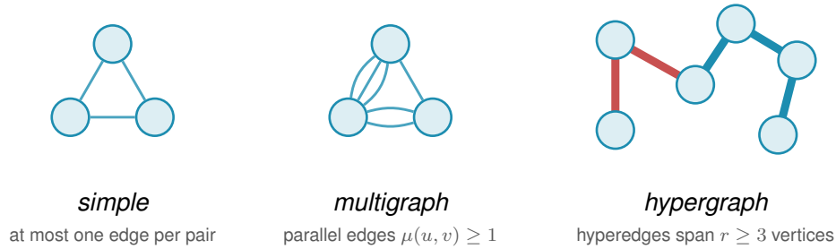
Figure 1.3. The first axis of variation, the model . In a simple graph each pair of vertices is joined by at most one edge. A multigraph permits parallel edges, here a triple and a double, so the multiplicity \mu(u, v) counts how many copies join a pair. A hypergraph replaces pairwise edges by hyperedges, drawn here the way a metro map draws lines: the red line threads three vertices and the blue line threads four, and they meet at the single station they share, illustrating hyperedges of different sizes that may overlap. When all hyperedges have the same size r we call it an r -uniform hypergraph. The same connectivity question, how many independent routes a pair can be forced to share, is asked of all three.
