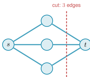
Figure 1.2. Menger's theorem in miniature. Between s and t run three routes that share no edge, so \lambda(s, t) = 3 . Removing the three edges that enter t (red dashed) cuts every route, and no two edges can, so the smallest separating set also has size three. The most independent routes a pair can muster always equals the cheapest cut between them, the fact every bound in this thesis leans on.
