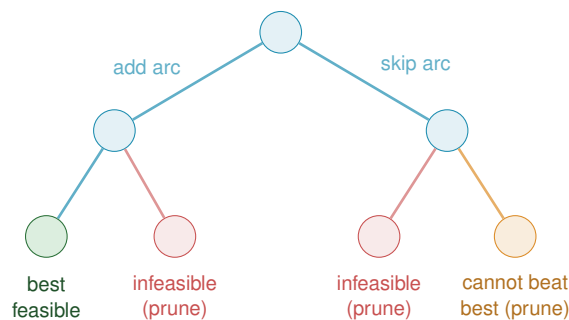
Figure 2.7. Branch and bound over digraphs. Each node fixes one more cell, arc present or absent, so the leaves are whole digraphs. Two rules cut entire subtrees before they are walked. A branch whose partial digraph already breaks the connectivity ceiling is infeasible, and so is every completion of it (red). A branch whose best possible completion still cannot beat the densest feasible digraph found so far is dropped on the counting bound (orange). Only the surviving branches are explored, which is what lets the search reach the base cases n \leq 7 the blind walk cannot.
