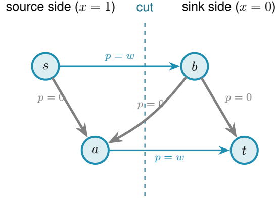
Figure 2.9. One ordered pair’s chosen cut. The dashed line splits the vertices into the source side, where x_u^{st} = 1 , and the sink side, where x_u^{st} = 0 . Only arcs running from source side to sink side cross the cut, and the first constraint forces their helper p_{uv}^{st} up to the arc weight w (the two thick arcs). Arcs that stay on one side, and arcs that run the other way across the line, contribute nothing. The second constraint then caps the total counted weight, the thick arcs, at one.
