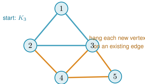
Figure 1.6. A 2-tree grown one vertex at a time. The blue triangle on \{1, 2, 3\} is the starting K_3 . Vertex 4 is then joined to the two ends of the edge \{2, 3\} , and vertex 5 to the two ends of the edge \{3, 4\} (orange edges), each new vertex hung on an edge already present. A general k -tree follows the same recipe with K_{k+1} in place of the triangle and a k -clique in place of the edge. These are the chordal scaffolds Leonard’s count rests on.
