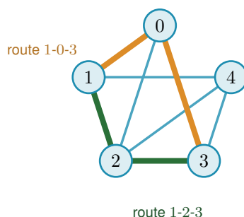
Figure 1.1. A simple graph on five vertices. It is K_5 , the complete graph in which every one of the \binom{5}{2} = 10 pairs is joined by an edge, with the two edges \{0, 4\} and \{1, 3\} removed, so its edge set E(G) holds eight edges. The five dots are the vertex set V(G) and the lines are the edges. The pair 1, 3 carries no edge of its own, yet it still has two routes that share no edge, 1-0-3 (orange) and 1-2-3 (green), so its local edge-connectivity, defined just below, is \lambda(1, 3) = 2 . Since at most one line joins any given pair and no edge loops back to its own endpoint, this is a simple graph.
