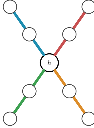
Figure 1.12. The star hypertree that attains the m = 2 hypergraph bound, here r = 3 and n = 9 , drawn as a metro map. The single hub station h lies on every line, and each of the \lfloor (n-1)/(r-1) \rfloor = 4 hyperedges is one metro line of r = 3 stations that hangs a fresh block of r-1 = 2 vertices off the hub. Because every line meets every other only at h , no pair has two hyperedge-disjoint routes, so the Berge connectivity is one everywhere, exactly as a spanning tree attained the multigraph bound.
