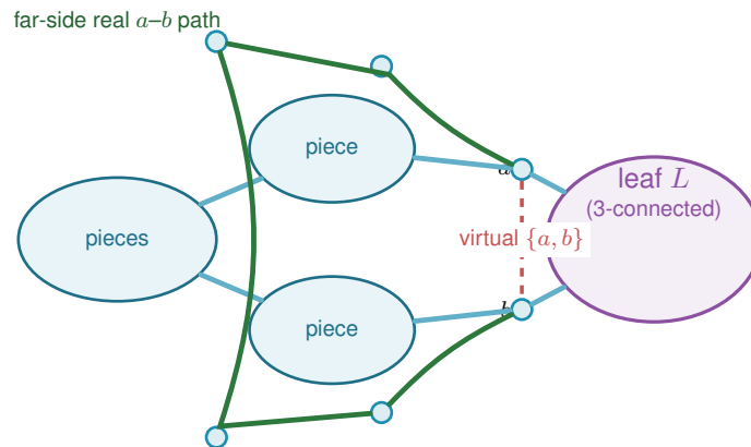
Figure A.7. The triconnected (Tutte/SPQR) decomposition in Step 4 of Lemma A.36, schematic: G splits into a tree of pieces (blobs) glued along virtual edges, and the analysis works at a leaf L with its single virtual edge \{a, b\} (dashed red). The far side of the tree supplies a real a – b path (green) that internally avoids L . If L is 3-connected, any two of its vertices are joined by three internally disjoint paths inside L , at most one using the virtual edge, and the far-side path replaces it, so \kappa_G \geq 3 for every pair in L . With |V(L)| \geq 4 that forces a hyperedge-node z^* \notin \{a, b\} of degree at most one, which is the contradiction that closes the lemma.
