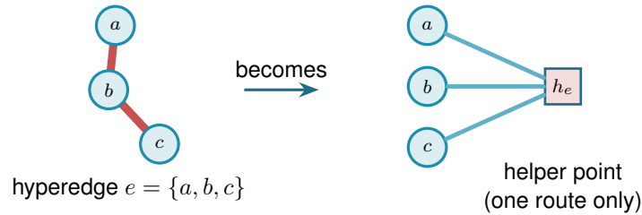
Figure 2.5. Measuring Berge connectivity by maximum flow. A hyperedge e , drawn as a metro line through its members (left), is replaced by a helper point h_e joined to each member (right). Because at most one route may pass through h_e , the line runs one train at a time, so the hyperedge serves only one route. Counting independent routes between two vertices is then an ordinary maximum flow on this enlarged network, and a two-vertex hyperedge collapses to a single ordinary edge.
