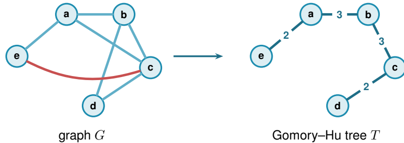
Figure A.1. A simple graph G (left) and a Gomory–Hu tree T of it (right); both live on the same five vertices, and here T is the path e-a-b-c-d with the marked cut weights. The four edges ea, ab, bc, cd are also tree edges, so each has \text{dist}_T(e) = 1 : these are the E_1 edges of Lemma A.4 , and a simple graph admits at most n - 1 = 4 of them, one per tree edge. The edges ac and bd join tree-distance-2 pairs, and the red chord ec has \text{dist}_T(ec) = 3 , crossing all three cuts on the path e-a-b-c . Reading \text{dist}_T(e) as the number of tree cuts an edge crosses makes \sum_e \text{dist}_T(e) = \sum_t c(t) ( Lemma A.6 ); every edge crosses at least one cut, but only the n - 1 tree edges cross exactly one, which is the surplus that drives Lemma A.5 and ultimately the factor of two in Mader’s bound.
