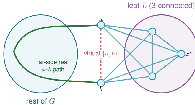
Figure A.6. The triconnected (Tutte/SPQR) decomposition in Step 4 of Lemma A.48, schematic: G splits into a tree of pieces (blobs) glued along virtual edges, and the analysis works at a leaf L with its single virtual edge \{a, b\} (dashed red). The far side of the tree supplies a real a – b path (green) that internally avoids L . If L is 3-connected, any two of its vertices are joined by three internally disjoint paths inside L , at most one using the virtual edge, and the far-side path replaces it, so \kappa_G \geq 3 for every pair in L . With |V(L)| \geq 4 that forces a hyperedge-node z^* \notin \{a, b\} of degree at most one, which is the contradiction that closes the lemma.
