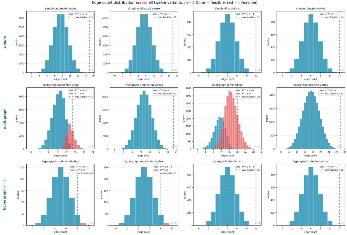
Figure B.7. The same enumeration at m = 6 viewed by edge count, the companion to Figure 4.5. Feasible graphs are blue, infeasible ones red, and the dotted vertical line marks the extremal value at that size. File edges_dist_m6.png.
