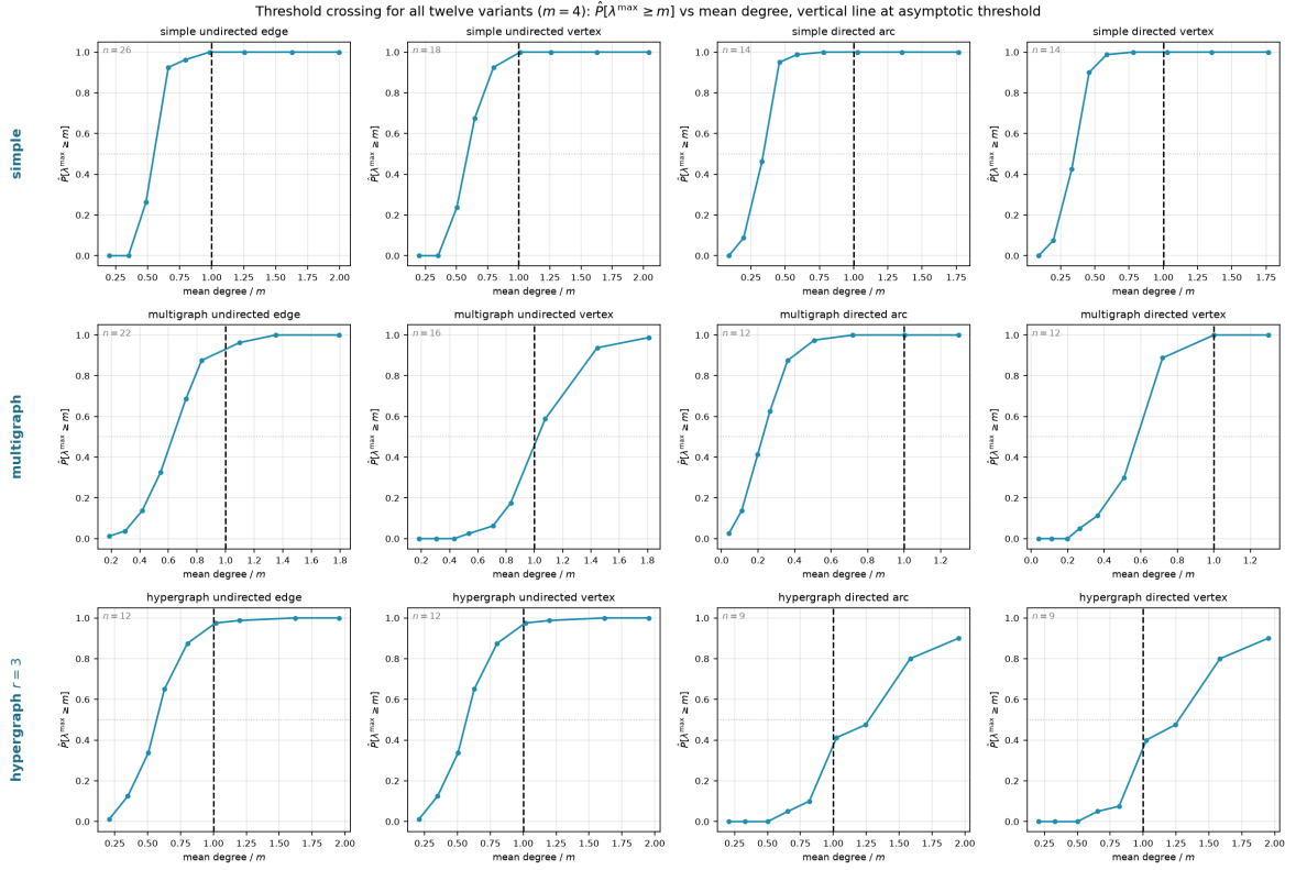
Figure 4.3. Threshold-crossing curves for all twelve variants at m = 4 , one panel per variant. Each panel plots \hat{P}[\lambda^{\max} \geq m] against the measured mean binding degree in units of m ; the vertical dashed line marks the asymptotic threshold degree = m of Theorem 1.15 . The six-way model ordering of Figure 4.2 is visible within each separation type: directed panels cross the line with less degree than their undirected counterparts, and hypergraph panels cross last. Per-panel n is annotated. Multigraph panels use the hurdle-geometric model with \alpha = \frac{1}{2} , multiplicities capped at m - 1 .
