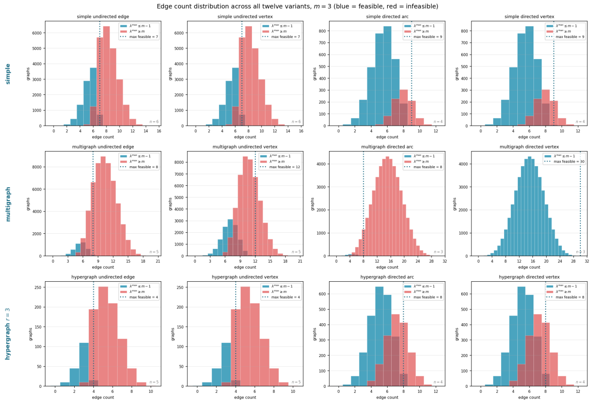
Figure 4.5. The same enumeration viewed by edge count rather than connectivity, at m = 3 . Feasible graphs are blue, infeasible ones red. The dotted vertical line marks the largest feasible edge count, the extremal value at this n read straight from the full enumeration, so the reader can see directly how far the extremal graphs sit from the bulk of the distribution and whether the extremal density is typical or exceptional.
