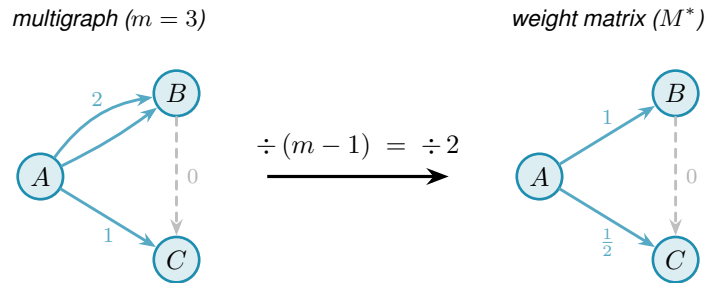
Figure 2.7. Scaling at m = 3 : dividing multiplicities by m-1 = 2 turns the integer multigraph into a weight matrix with entries in [0, 1] and pairwise maximum flow at most one. Hence one m -free optimisation bounds every threshold.
