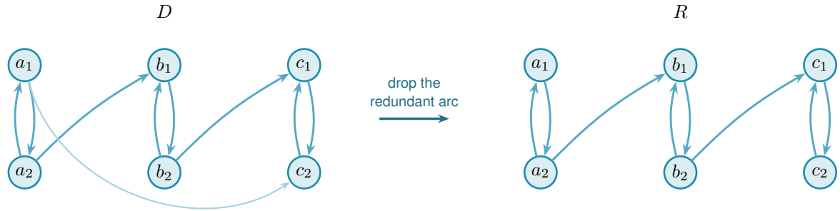
Figure A.2. A small instance of Lemma A.19 . In D (left) three bidirected pairs A = \{a_1, a_2\} , B = \{b_1, b_2\} , C = \{c_1, c_2\} are the strongly connected components, joined by a_2 \rightarrow b_1 , b_2 \rightarrow c_1 , and a_1 \rightarrow c_2 . Contracting each pair to a point gives a condensation Q_0 on three points, carrying all three arcs A \rightarrow B , B \rightarrow C and A \rightarrow C . That is exactly the transitively-closed triangle the proof rules out of the thinned Q . The arc A \rightarrow C is redundant, since A already reaches C through B , so the transitive reduction Q keeps only A \rightarrow B and B \rightarrow C . The underlying graph of Q is then a path on three points, triangle-free as claimed. The reachability skeleton R (right) reflects exactly this: every SCC keeps both of its internal arcs (an in- and an out-arborescence on two vertices is just the pair itself), while of the three component-crossing arcs of D only the two witnesses of Q 's two arcs survive. The direct arc a_1 \rightarrow c_2 is dropped, yet a_1 still reaches c_2 in R : first a_1 \rightarrow a_2 , then a_2 \rightarrow b_1 , then b_1 \rightarrow b_2 , then b_2 \rightarrow c_1 , then c_1 \rightarrow c_2 .
