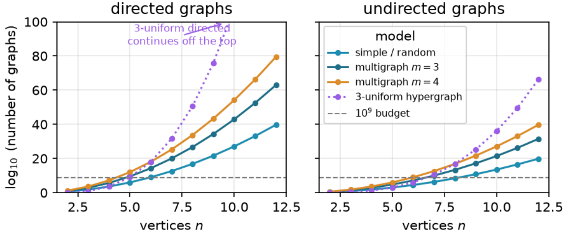
Figure 2.8. Candidate counts for blind enumeration on a logarithmic scale. Every model crosses the generous 10^9 budget in single-digit order, and directed objects grow fastest because they have more independent cells to fill.
