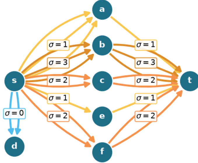
Figure 2.9. Arc sensitivity in a directed multigraph with \lambda^{\max} = 9 . Equal multiplicities can have different \sigma : the downstream bottleneck makes s \rightarrow a cooler than s \rightarrow b , while arcs into the dead end d have \sigma = 0 .
