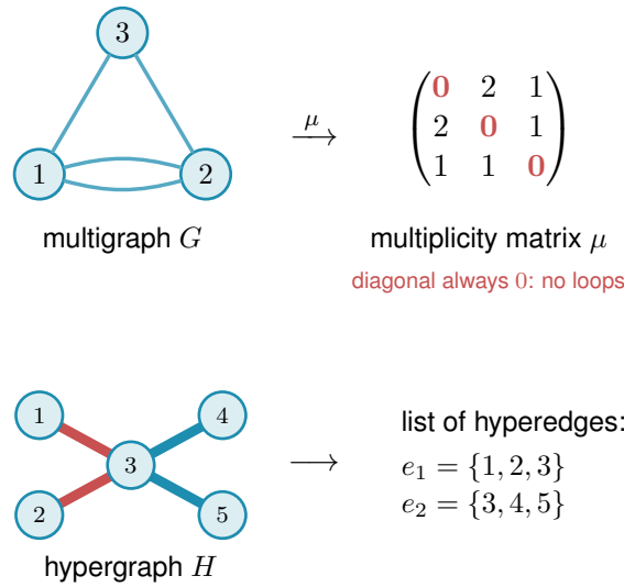
Figure 2.4. The two encodings. A graph or digraph is the multiplicity matrix \mu , which is symmetric when undirected and binary when simple. A hypergraph is a list of vertex sets instead, since a matrix would need n^r entries and be almost all zero. A multihypergraph repeats an entry in that list.
