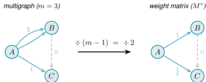
Figure 2.6. Scaling at m = 3 : dividing multiplicities by m - 1 = 2 turns the integer multigraph into a weight matrix with entries in [0, 1] and pairwise maximum flow at most one. Hence one m -free optimisation bounds every threshold.
