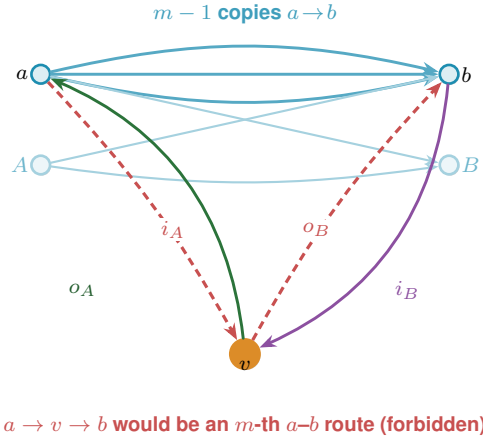
Figure A.4. The attachment lemma (Lemma A.33): a new vertex v is glued onto (m-1) \cdot B_{p,q} , the one-directional complete bipartite multigraph in which every a \in A sends m-1 parallel arcs to every b \in B (the bundle along the top, faint for the pairs other than a, b ). The arcs at v fall into four classes by direction and side: i_A into v from A , o_A out of v to A , i_B into v from B , and o_B out of v to B . The two red legs i_A and o_B are drawn together because they are the worst case: the route a \rightarrow v \rightarrow b laid on top of the m-1 existing a \rightarrow b arcs is an m -th arc-disjoint a - b route, so \lambda(a, b) \geq m , which feasibility forbids. Ruling this out, with two siblings like it, caps d(v) \leq (m-1)\max(p, q) .
