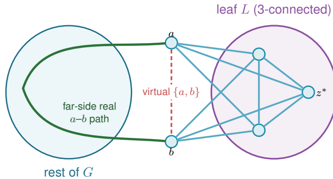
Figure A.7. The triconnected (Tutte/SPQR) decomposition in Step 4 of Lemma A.46 , schematic: G splits into a tree of pieces (blobs) glued along virtual edges, and the analysis works at a leaf L with its single virtual edge \{a, b\} (dashed red). The far side of the tree supplies a real a – b path (green) that internally avoids L . If L is 3-connected, any two of its vertices are joined by three internally disjoint paths inside L , at most one using the virtual edge, and the far-side path replaces it, so \kappa_G \geq 3 for every pair in L . With |V(L)| \geq 4 that forces a hyperedge-node z^* \notin \{a, b\} of degree at most one, which is the contradiction that closes the lemma.
