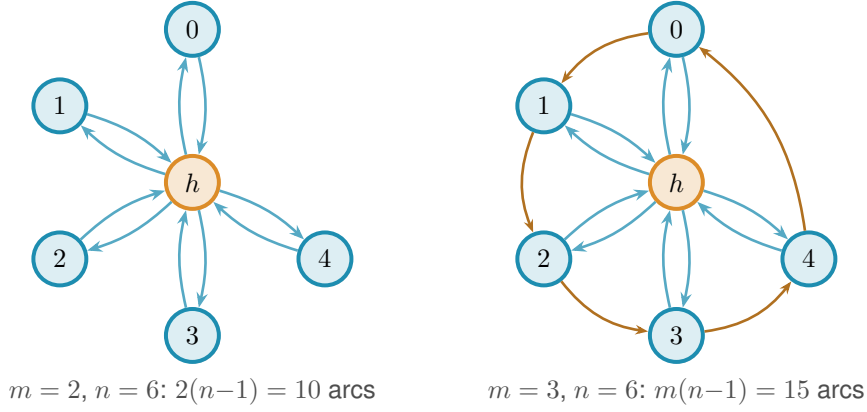
Figure 1.9. The directed hub at n = 6 for two values of m . Left ( m = 2 ): the bidirected star. The hub h is joined to each spoke by one arc in each direction, giving 2(n - 1) = 10 arcs. No circulant layer is added, so all spoke communication routes through h , so \lambda^{\max} = 1 . Right ( m = 3 ): a single circulant layer is added among the five spokes. The blue arcs are the same hub-spoke pairs as on the left. The orange arcs are that one circulant layer, the cycle 0 \rightarrow 1 \rightarrow 2 \rightarrow 3 \rightarrow 4 \rightarrow 0 , so each spoke has d^+ = d^- = m - 1 = 2 . The total is m(n - 1) = 15 arcs and \lambda^{\max} = 2 . For m \geq 3 the spokes are no longer isolated from one another, and tracing all the routes becomes the argument that fills the rest of the chapter.
