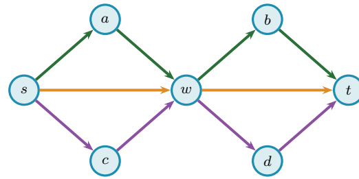
(a) original digraph
