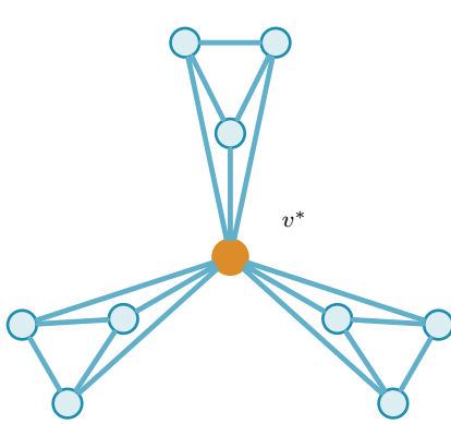
(a) Shared-clique graph: three K_4 's glued at one hub v^* ( m = 4 , k = 3 ). Each non-hub vertex has degree m-1 = 3 .
