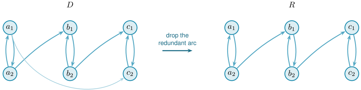
Figure A.2. The construction of Lemma A.19. Each bidirected pair A, B, C is a strongly connected component. Contracting the pairs gives A \rightarrow B \rightarrow C and the redundant arc A \rightarrow C . Delete that arc to obtain the triangle-free transitive reduction. The skeleton R keeps the internal arcs of each pair and the two remaining connections between pairs. Although a_1 \rightarrow c_2 is removed, a_1 still reaches c_2 through B .
