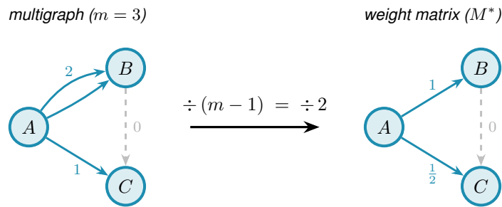
Figure 2.7. The scaling step for m = 3 . Dividing each multiplicity by m-1 = 2 maps the integer multigraph (left) to a weight matrix with all values in [0, 1] and max-flow at most one between every pair (right). The double arc A \rightarrow B (multiplicity 2) becomes weight 1, the single arc A \rightarrow C (multiplicity 1) becomes weight \frac{1}{2} , and the absent arc B \rightarrow C (multiplicity 0, shown dashed) stays absent. Crucially, m drops out on the right, so a single optimisation over all weight matrices pins L_m^{\text{dir}}(n) = (m-1) M^*(n) for every m simultaneously.
