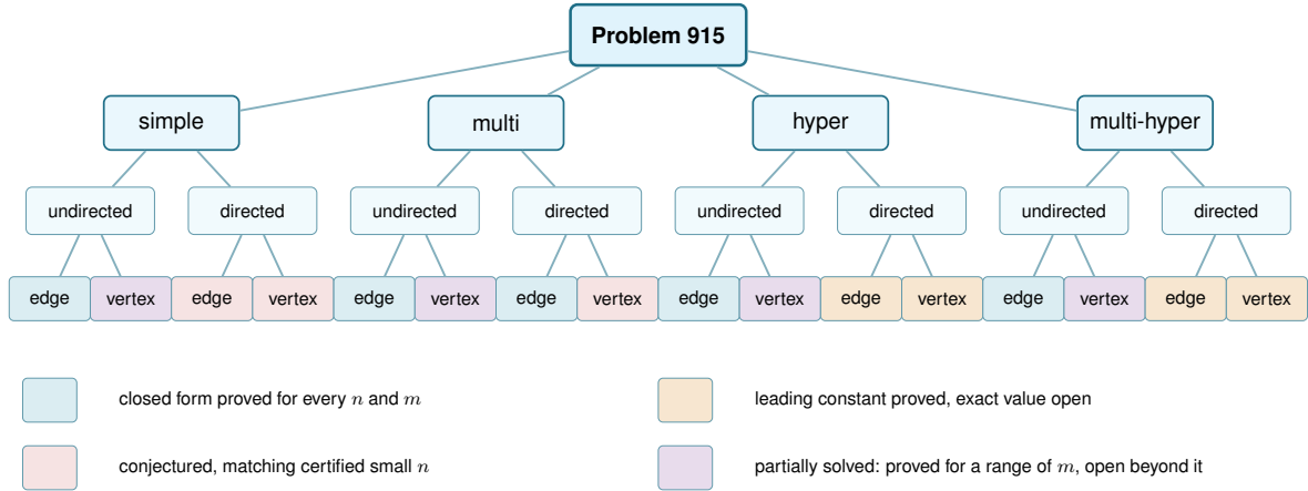
Figure 3.3. Status of the sixteen variants. Colour marks the status of a leaf: blue a closed form proved for every n and m , purple a value proved for a range of m and open beyond it, red a conjectured exact formula with a proved lower bound, and amber a proved leading term with the exact value unknown. The model and direction rows are labels and carry no status, since each of them now covers two leaves that differ. Table 3.1 is authoritative for exceptions and conventions.
