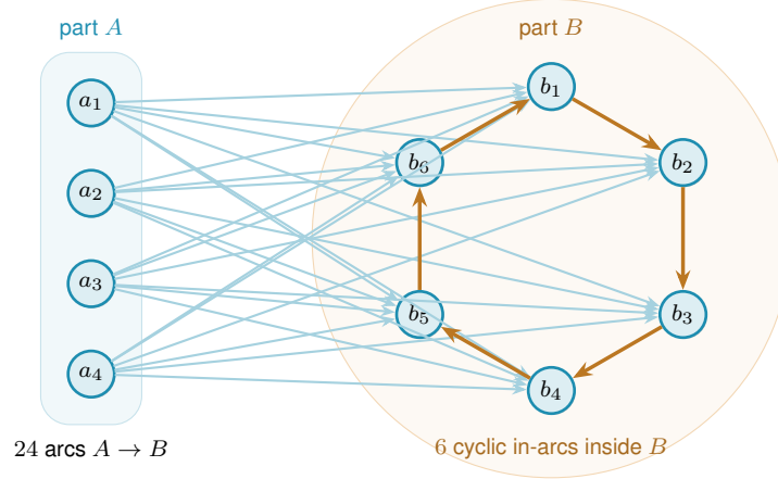
Figure 3.2. The augmented bipartite digraph of Construction A.17 at m = 3 , n = 10 . Every arc runs from A to B , and inside B each vertex takes one arc from its cyclic predecessor, which is m - 2 arcs per vertex. A pair a_i, b_j then has the direct arc and one detour, so \lambda^{\max} = 2 , and the count is 24 + 6 = 30 against the hub branch's 27.
