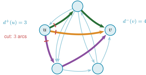
Figure 1.4. A directed version of the K_5 example with multiple arcs. Three arc-disjoint directed routes connect u to v (orange, green, purple). The three red marks cut the arcs leaving u , the first arc of each route, so \lambda(u, v) = 3 by Menger's theorem. A directed cut counts only the arcs leaving u 's side, so the lone arc entering u from the top is not part of it. The out-degree d^+(u) = 3 and in-degree d^-(v) = 4 bound the value from above, and \lambda(u, v) = \min(3, 4) = 3 meets the smaller one, at u .
