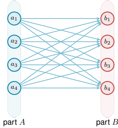
Figure 1.8. The one-directional complete bipartite digraph B_{k,k} of Construction 1.7 , drawn here at n = 8 with |A| = |B| = 4 . Every one of the |A| \cdot |B| = \lfloor n^2/4 \rfloor arcs runs left to right, from A to B . There are no arcs inside A , inside B , or back from B to A . Because B has no outgoing arcs and A no incoming ones, the only route from any a_i to any b_j is the single arc a_i \rightarrow b_j , so every pair has local edge-connectivity 1 while the arc count grows quadratically.
