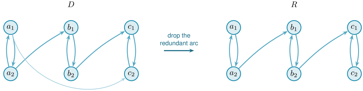
Figure A.4. A small instance of Lemma A.36 . In D (left) three bidirected pairs A = \{a_1, a_2\} , B = \{b_1, b_2\} , C = \{c_1, c_2\} are the strongly connected components, joined by a_2 \rightarrow b_1 , b_2 \rightarrow c_1 , and a_1 \rightarrow c_2 . Contracting each pair to a point gives a condensation Q_0 on three points, with all three arcs A \rightarrow B , B \rightarrow C , A \rightarrow C present, exactly the transitively-closed triangle the proof rules out of the thinned Q : the arc A \rightarrow C is redundant, since A already reaches C via B , so the transitive reduction Q keeps only A \rightarrow B and B \rightarrow C , and the underlying graph of Q , a path on three points, is triangle-free as claimed. The reachability skeleton R (right) reflects exactly this: every SCC keeps both of its internal arcs (an in- and an out-arborescence on two vertices is just the pair itself), while of the two component-crossing arcs of D only the two witnesses of Q 's two arcs survive. The direct arc a_1 \rightarrow c_2 is dropped, yet a_1 still reaches c_2 in R : first a_1 \rightarrow a_2 , then a_2 \rightarrow b_1 , then b_1 \rightarrow b_2 , then b_2 \rightarrow c_1 , then c_1 \rightarrow c_2 .
