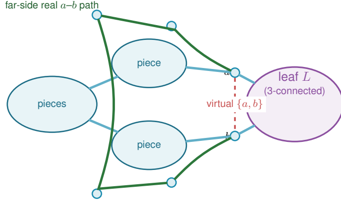
Figure A.7. The triconnected (Tutte/SPQR) decomposition in Step 4 of Lemma A.36 , schematic: G splits into a tree of pieces (blobs) glued along virtual edges, and the analysis works at a leaf L with its single virtual edge \{a, b\} (dashed red). The far side of the tree supplies a real a - b path (green) that internally avoids L . If L is 3-connected, any two of its vertices are joined by three internally disjoint paths inside L , at most one using the virtual edge, and the far-side path replaces it, so \kappa_G \geq 3 for every pair in L . With |V(L)| \geq 4 that forces a hyperedge-node z^* \notin \{a, b\} of degree at most one, which is the contradiction that closes the lemma.
