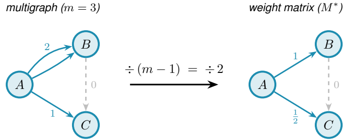
Figure 2.6. The scaling step for m = 3 . Dividing each multiplicity by m - 1 = 2 maps the integer multigraph (left) to a weight matrix with all values in [0, 1] and max-flow at most one between every pair (right). The double arc A \rightarrow B (multiplicity 2) becomes weight 1, the single arc A \rightarrow C (multiplicity 1) becomes weight \frac{1}{2} , and the absent arc B \rightarrow C (multiplicity 0, shown dashed) stays absent. Crucially, m drops out on the right, so a single optimisation over all weight matrices pins L_m^{\text{dir}}(n) = (m - 1) M^*(n) for every m simultaneously.
