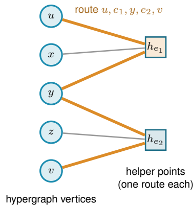
Figure 2.5. The same construction on a two-hyperedge hypergraph e_1 = \{u, x, y\} , e_2 = \{y, z, v\} . The Berge route that enters e_1 at u , switches hyperedge at the shared vertex y , and leaves e_2 at v becomes the single flow path u \rightarrow h_{e_1} \rightarrow y \rightarrow h_{e_2} \rightarrow v (orange), entering each hyperedge through one member and leaving through another. Because each helper carries only one unit of flow, a second u-v route would have to avoid both helpers, which is exactly the rule that one hyperedge serves one route.
