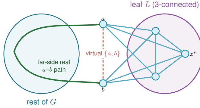
Figure A.6. The triconnected (Tutte/SPQR) decomposition in Step 4 of Lemma A.49 , schematic: G splits into a tree of pieces (blobs) glued along virtual edges, and the analysis works at a leaf L with its single virtual edge \{a, b\} (dashed red). The far side of the tree supplies a real a - b path (green) that internally avoids L . If L is 3-connected, any two of its vertices are joined by three internally disjoint paths inside L , at most one using the virtual edge, and the far-side path replaces it, so \kappa_G \geq 3 for every pair in L . With |V(L)| \geq 4 that forces a hyperedge-node z^* \notin \{a, b\} of degree at most one, which is the contradiction that closes the lemma.
